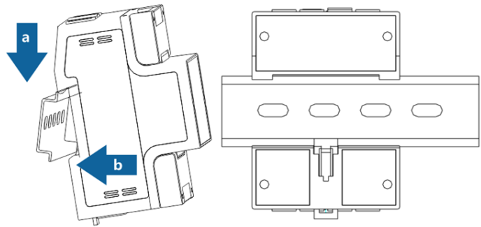
Figure 2-6 Meter Installation
