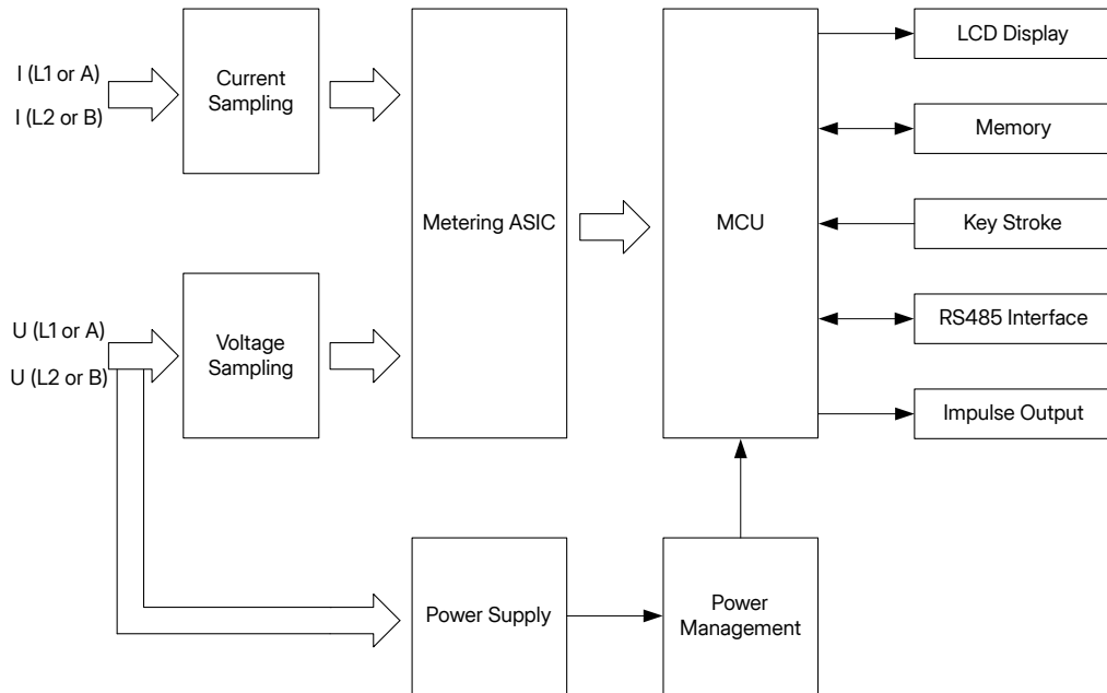
Figure 2-2 Working Principle Diagram
