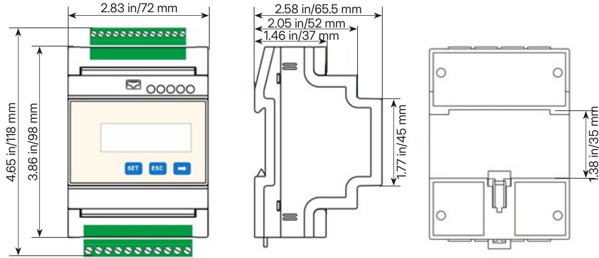
Figure 2-5 Product Dimensions
