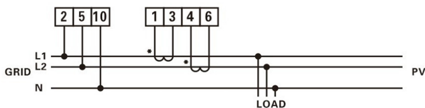
Figure 2-7 Type of Wiring 1P3W
