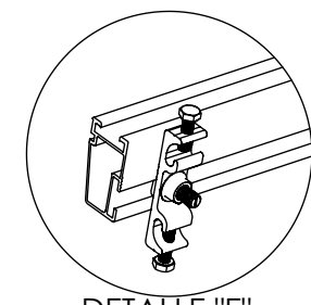
DETALLE "E" NXT-GC Terminal a Tierra
