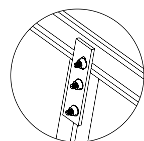
DETALLE "C" NXT-TILT Conector de riel RX
