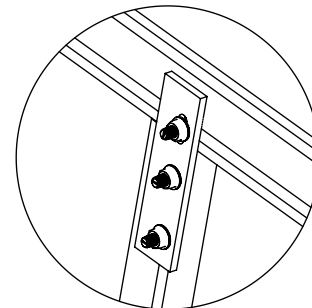
DETALLE "C" NXT-TILT Conector de riel RX
