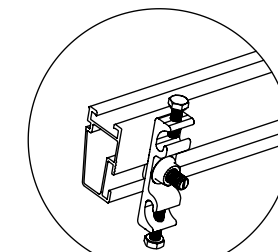
DETALLE "E" NXT-GC Terminal a Tierra
