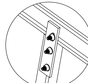
DETALLE "C" NXT-TILT Conector de riel RX
