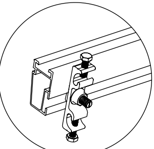
DETALLE "D" NXT-GC Terminal a Tierra
