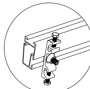
DETALLE "D" NXT-GC Terminal a Tierra
