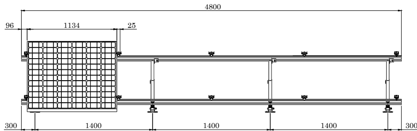
VISTA FRONTAL
