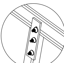
DETALLE "D" NXT-TILT Conector de riel RX
