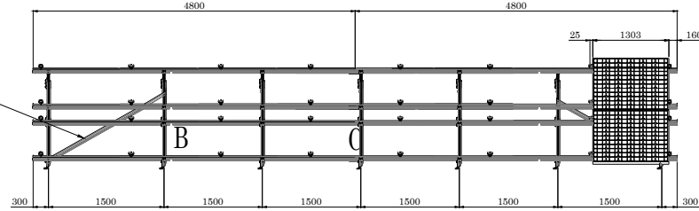
VISTA FRONTAL
