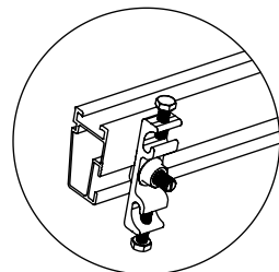
DETALLE "F" NXT-GC Terminal a Tierra
