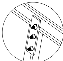
DETALLE "D" NXT-TILT Conector de riel RX
