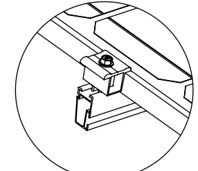
DETALLE "A" NXT-AUA Abrazadera Universal (Modo Remate)
