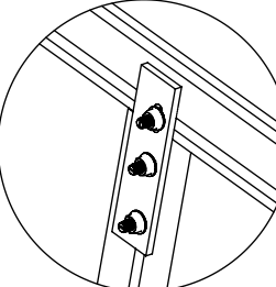
DETALLE "D" NXT-TILT Conector de riel RX
