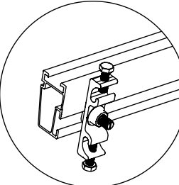
DETALLE "F" NXT-GC Terminal a Tierra
