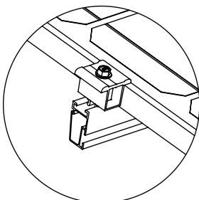
DETALLE "A" NXT-AUA Abrazadera Universal (Modo Remate)
