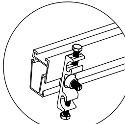
DETALLE "F" NXT-GC Terminal a Tierra
