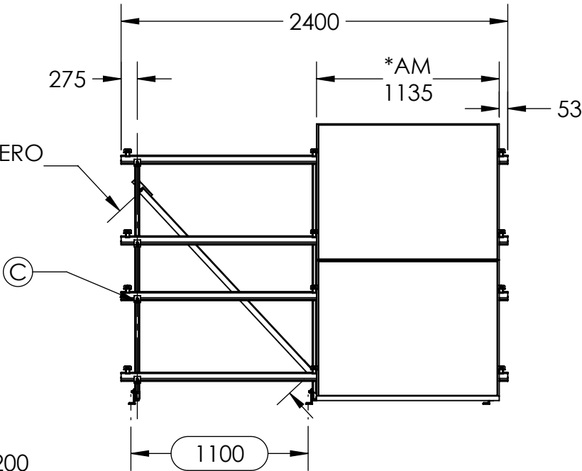
DETALLE "A" NXT-AUA Abrazadera Universal (Modo Remate)
