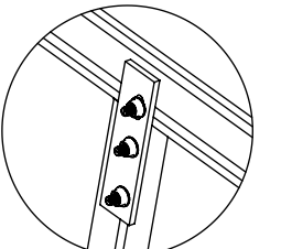
DETALLE "D" NXT-TILT Conector de riel RX
