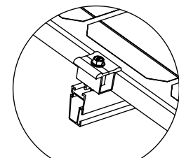
DETALLE "A" NXT-AUA Abrazadera Universal (Modo Remate)
