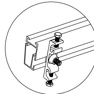
DETALLE "D" NXT-GC Terminal a Tierra
