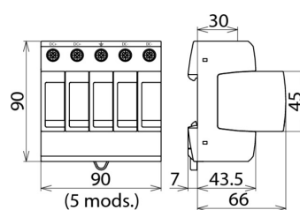
Dimension drawing DG M PV2 1200
