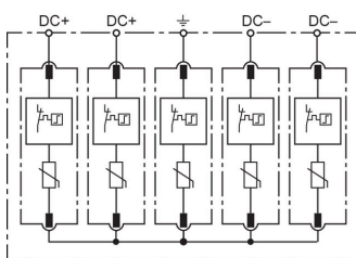
Basic circuit diagram DG M PV2 1200
