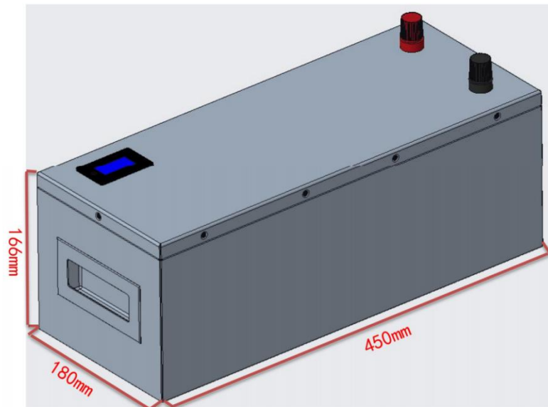
Dimension diagram (unit:mm)
